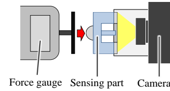
Figure 6. Schematic view of experimental setup for evaluating properties of sensing parts.
