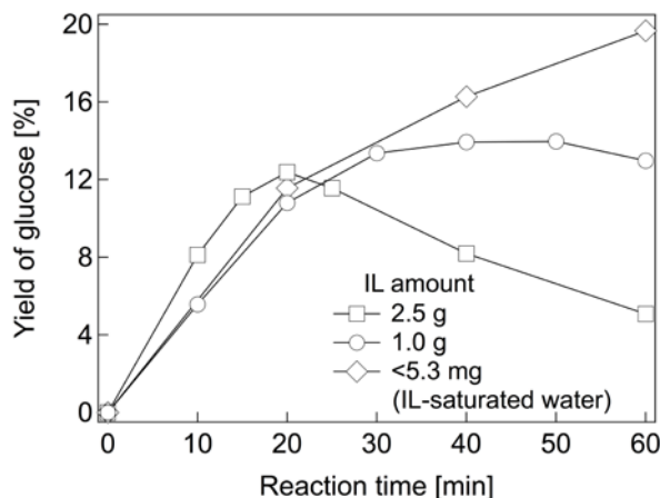
Figure 4. Time courses of glucose yield during hydrolysis of phosphoric acid-swollen cellulose with [P_{8,8,8,5}][HSO_4] /water biphasic systems and [P_{8,8,8,5}][HSO_4] -saturated aqueous solution under microwave heating at 190 °C. The biphasic systems consist of 2.5 or 1.0 g of [P_{8,8,8,5}][HSO_4] and 7.5 g of water.
