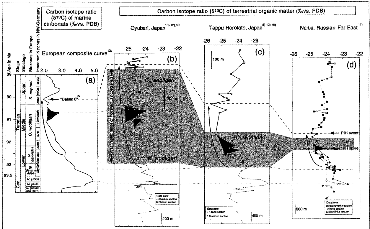
Fig. 2. Comparison of carbon isotope profiles for carbonate 13) and terrestrial organic matter from fore-arc basin sediments in Asia. 8),10),12),16),19) Correlative \delta^{13}C events are connected with broken lines. Shaded peaks indicate IH spike or the correlative carbon-isotopic event in Europe. See text for details.
