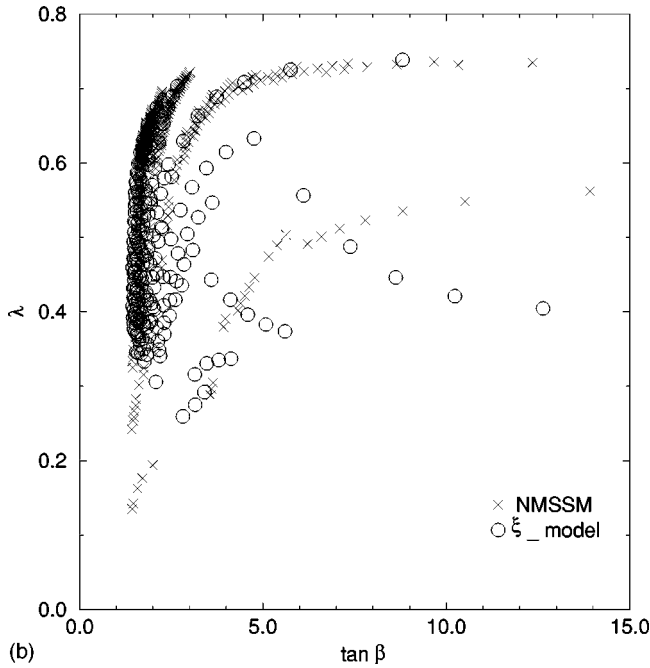
FIG. 2. Scatter plots of the radiative symmetry breaking solutions for the NMSSM and the \xi_- model in the (\tan\beta, \kappa or \kappa) plane (a) and the (\tan\beta, \lambda) plane (b). The values of \kappa , \kappa and \lambda are the ones at m_t .
