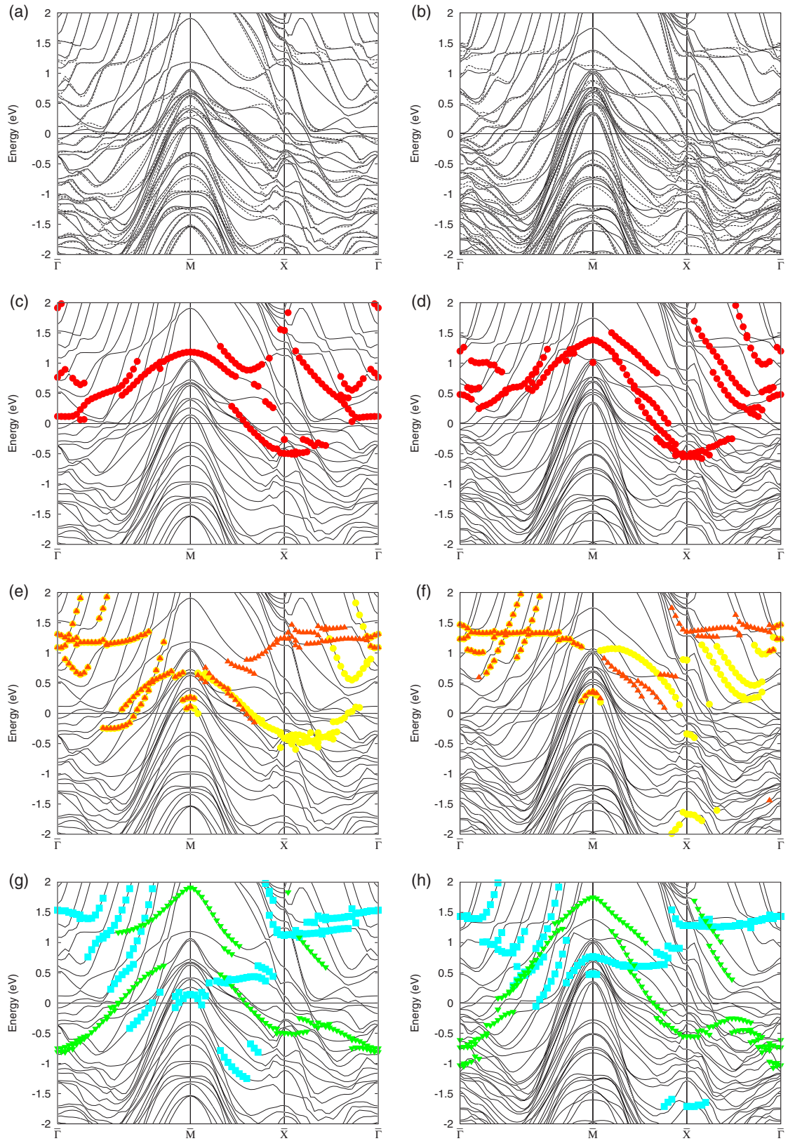
FIG. 2. (Color online) Band dispersions for the Fe/Pt(001) [(a), (c), (e), and (g)] and Pt/Fe/Pt(001) [(b), (d), (f), and (h)]. In the top panels, the magnetized direction dependence of the z axis (solid curves) and x axis (dashed curves) is shown. The Fe orbital local components of d_{3z^2-r^2} , d_{xz} , d_{yz} , d_{xy} , and d_{x^2-y^2} for minority spin states are marked as red circles, orange triangles, yellow circles, blue squares, and green triangles, respectively. See text for other details.
