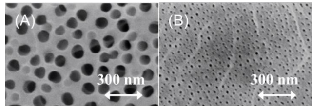
Fig. 2 SEM images of the surfaces of anodic alumina films prepared in oxalic acid bath (A) and sulfuric acid bath (B).
