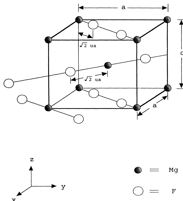
FIG. 1. Crystal structure of the tetragonal \text{MgF}_2 unit cell, where u is an atomic fractional coordinate.
