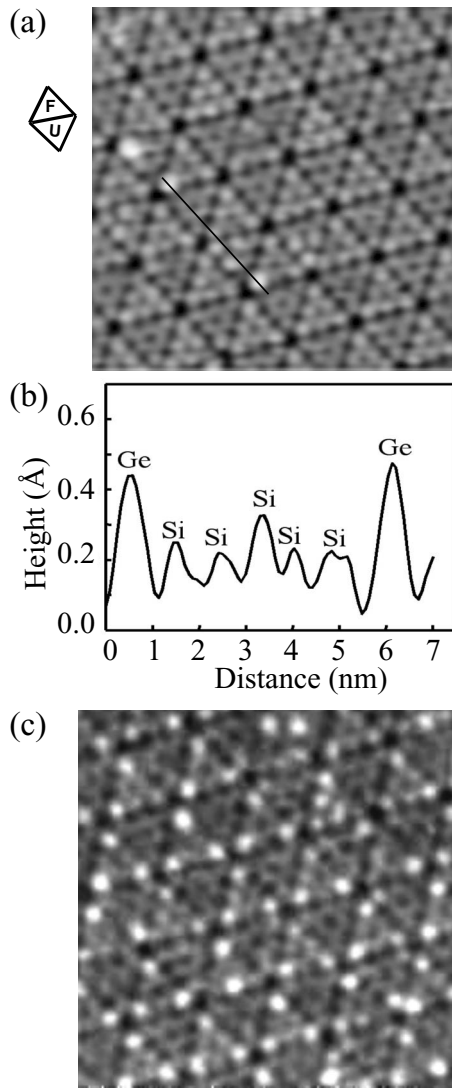
FIG. 1. STM images at RT with submonolayer Ge deposition on Si(111)- 7 \times 7 at 150^\circ\text{C} under a low flux of \sim 0.005 ML/min. (a) Filled state image of \sim 0.008 ML Ge; sample bias voltage ( V_s ) = -2.0 V, tunneling current ( I_t ) = 0.04 nA, and scan area: 15 \times 15 nm ^2 . (b) Line profile along a line in (a). (c) At 0.05 ML Ge, exhibiting a triangular pattern on each FHUC; V_s = -1.8 V and I_t = 0.04 nA.
