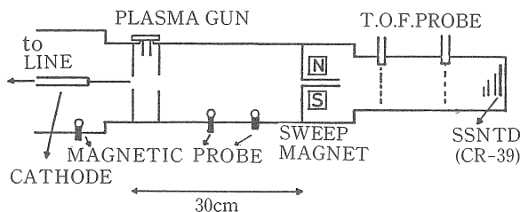
Fig. 1. A schematic diagram of the experimental apparatus.
