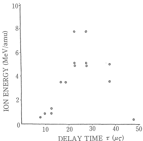
Fig. 3. Ion energy per amu vs. the delay time \tau .
