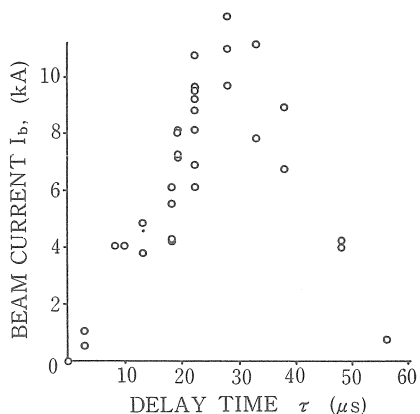
Fig. 4. Beam current at 10 cm downstream from the downstream side of the anode space.
