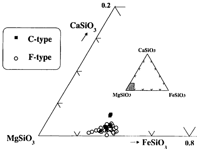
Fig. 6. Ca-Mg-Fe (total iron) atomic ratios of orthopyroxenes in the peridotite xenoliths from Iraya volcano, the Philippines.
