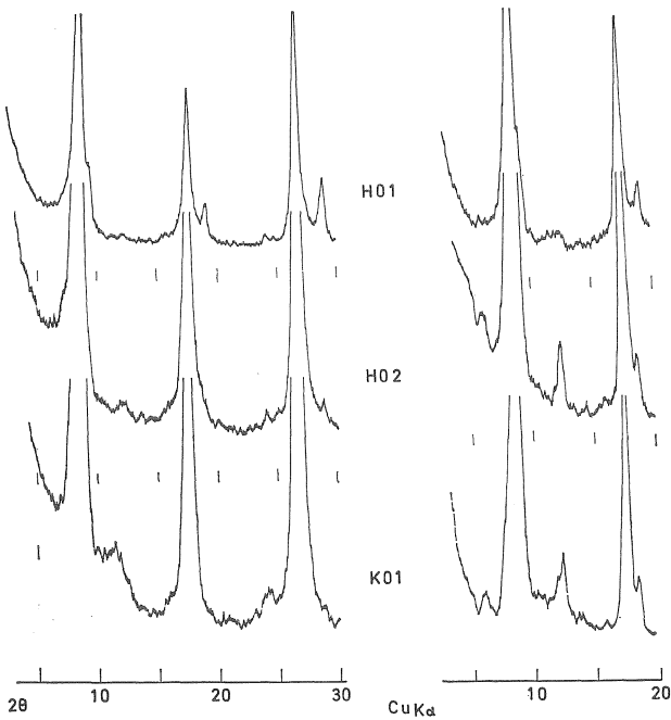
Fig. 3. X-ray diffraction patterns of oriented specimens after treatment of HCl and Ethylene Glycol of HO1, HO2 and KO1 left : HCl treatment right: Ethylene Glycol treatment
