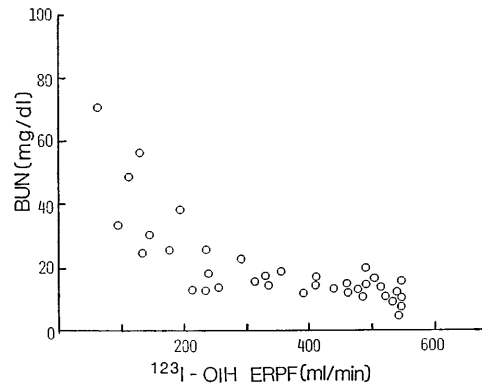
Fig. 3 Correlation between 123 I-OIH ERPF and BUN.
