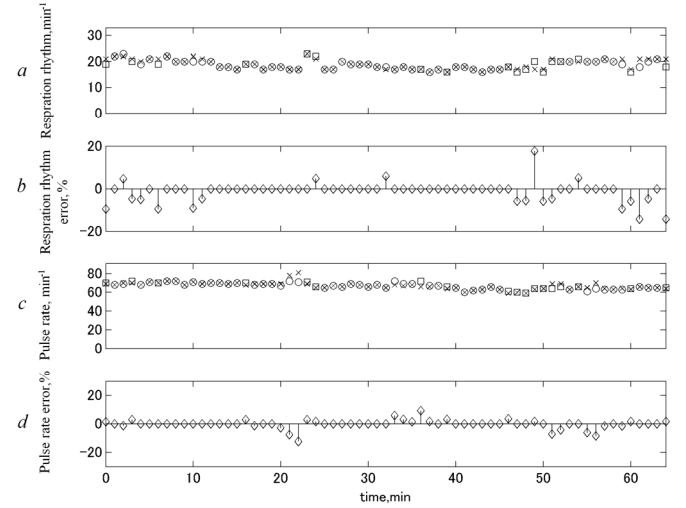
Fig. 5 Instantaneous profiles of (a) respiration rhythm and (c) pulse rate detected from the extracted waveforms (○ or □) and the reference data (×); and estimation errors of (b) respiration rhythm and (d) pulse rate. ○ indicates the value is detected when there is no artifact at that minute. □ indicates there are artifacts at that minute and the value shown is the average respiration rhythm or pulse rate estimated from the artifact-free signal at that minute.
