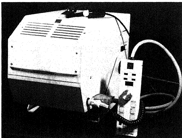
Fig. 2. Photograph of the portable device to measure the contrast threshold for motion perception (CTMP).
