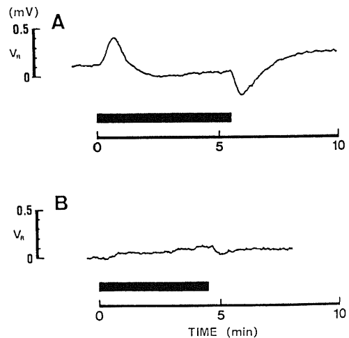
Fig. 12. Changes in the trans-retinal potential ( V_R ) induced by raising [HCO 3 - ] in isolated cat retina. [HCO 3 - ] was raised by 20 mM (black horizontal bar). Responses in A and B were recorded from the same preparation. An increase of [HCO 3 - ] in the vitreous side increased V_R transiently (A), while an increase of [HCO 3 - ] in the receptor side had almost no effect on V_R (B).
