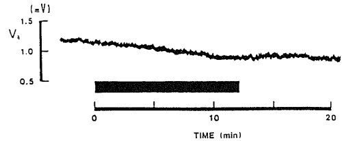
Fig. 11. The potential response from the excised anterior segment of cat eye to an increase of [HCO 3 - ]. The potential was recorded between the corneal side and the vitreous side ( V_a ) of the anterior segment. [HCO 3 - ] was increased by 20 mM (black horizontal bar) in the vitreous side.
