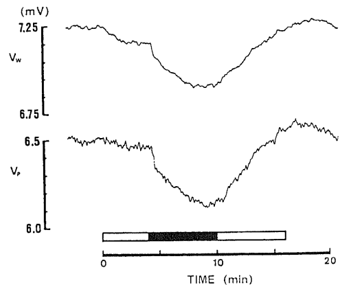
Fig. 6. Responses of V_w and V_p to an intravenous injection of 1.4% \text{NaHCO}_3 solution in the cat. Lactate Ringer's solution was injected at a rate of 0.56 ml/min/kg (white horizontal bar) before and after 1.4% \text{NaHCO}_3 injection (black horizontal bar) at the same rate. V_w (upper record) and V_p (lower record) decreased after 1.4% \text{NaHCO}_3 injection. The amplitude of V_p was approximately 1.25 times larger than that of V_w .
