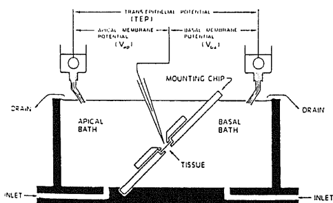
Fig. 3. Diagram of the perfusion chamber used for intracellular recordings. The mounting chip consisted of two plates, each of which had a 3 mm centered circular hole. The two sides of the tissue, apical surface of retinal pigment epithelium (RPE) vs. choroid, hereafter called basal surface, were immersed in 3.0 ml baths separately perfused at a rate of 10 ml/min.
