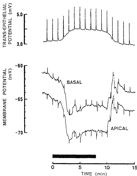
Fig.14. Changes in the TEP and membrane potentials of the RPE cell induced by raising apical [HCO 3 - ] in the cat RPE-choroid. Apical [HCO 3 - ] was raised by 20 mM (black horizontal bar). V ba was superimposed on V ap by the amplitude of TEP.
