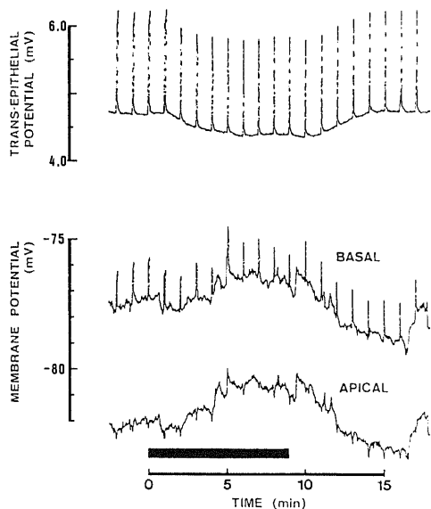
Fig.13. Changes in the TEP and membrane potentials of the RPE cell induced by raising basal [HCO 3 - ] in cat RPE-choroid. Basal [HCO 3 - ] was raised by 20 mM (black horizontal bar). The basal membrane potential (V ba ) was superimposed on apical membrane potential (V ap ) by the amplitude of TEP. Spiky deflections were produced by extrinsic trans-epithelial current pulses (1μA, 3 sec).
