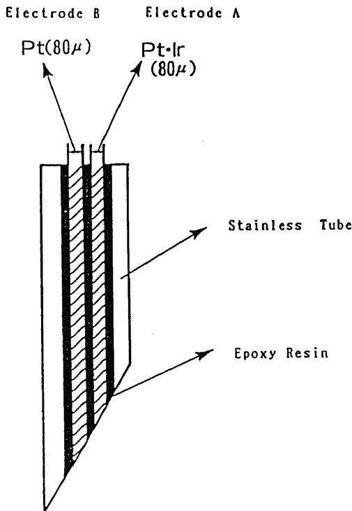
Fig.1. Schematic presentation of the bipolar electrode. The outer diameter of the stainless tube is 450 μ and the inner diameter is 230 μ.
