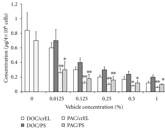
FIGURE 7: Effects of surfactants on uptake of paclitaxel and docetaxel in AH130 cells. Cells were treated with 3 µg/mL of docetaxel (DOC) or paclitaxel (PAC) dissolved with 0.125% ethanol (0) or the indicated concentrations of crEL or PS-80 (PS) for 30 min. The data at 0.0125% concentration of these surfactants are taken from [15]. Each column with bar represents the mean ± SD of at least three experiments performed in triplicate. *,**Significantly different from docetaxel at P < 0.05 and 0.01, respectively.
