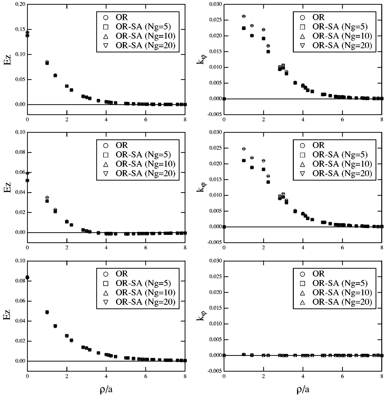
FIG. 3. The same plot as in Fig. 2 at \beta=2.4 for W(4,4) .
