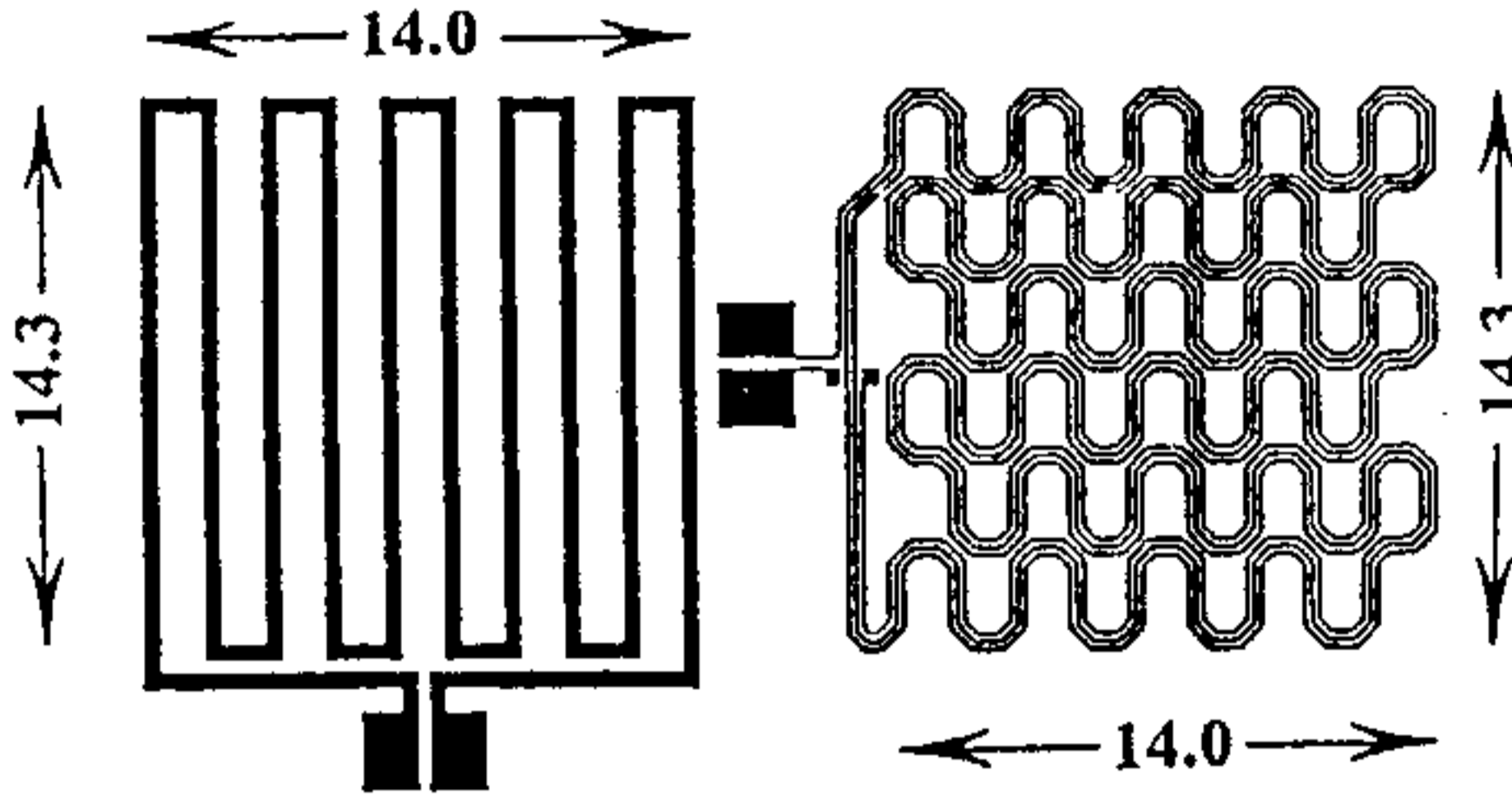
Width:0.5, Coil pitch:1.0 Width: 0.1, Coil pitch:0.1 Thickness:0.012mm Thickness:0.012mm, N=3turns (a) Meander coil (b) Mesh coil
