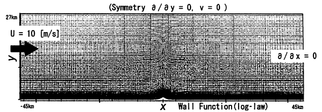
Fig. 1 Computational domain and boundary conditions
