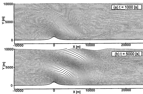
Fig. 2 Stream lines in the one-layer model for Fr = 1.0 . (a) t = 1000 \text{ [s]} , (b) t = 5000 \text{ [s]}
