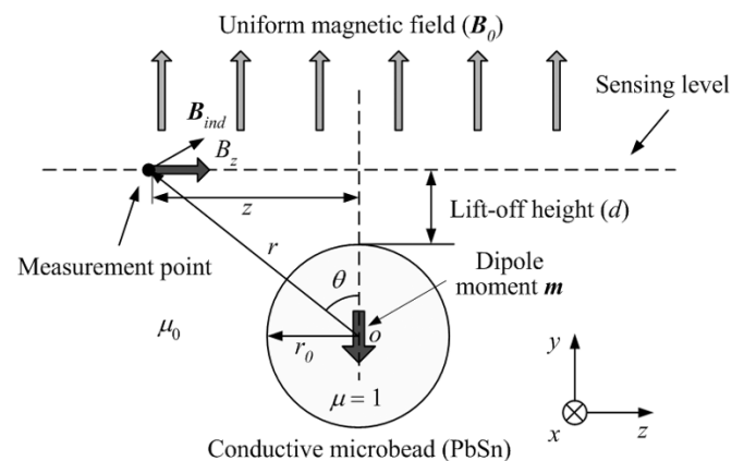
Fig. 2. Analytical model.
