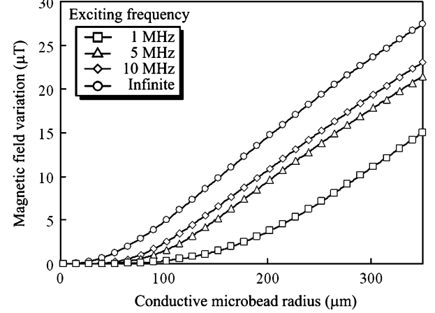
Fig. 5. Maximum magnetic field variation vs. conductive microbead (PbSn) radius obtained from analytical solution where lift-off height is 162 \mu\text{m} .
