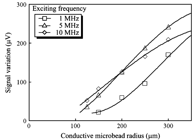
Fig. 7. Maximum signal variation vs. conductive microbead (PbSn) radius obtained from the experiment.
