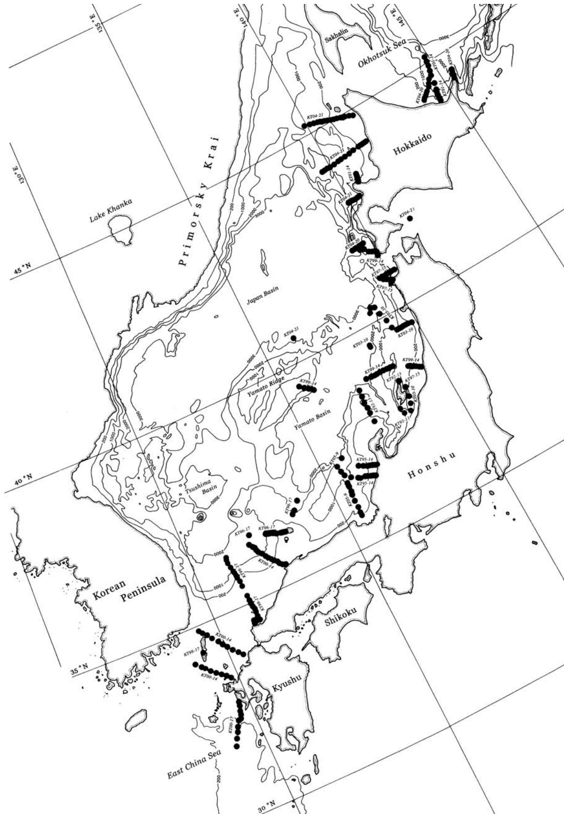
Fig.1 Localities of all submarine surface sediment samples in the Japan Sea and the surrounding seas collected by R/V Tansei-mar and Kanazawa University from 1995 - 2005 (samples of KT92-13 in 2003 are included; based on Geographical Survey of Japan 2003).
