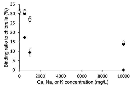
Fig 4. Adsorption of 85 Sr to Chlorella in the presence of cations. Binding ratios of 85 Sr to Chlorella in the presence of Na + (closed circles), K + (open circles), or Ca 2+ (closed diamonds). Data are expressed as the mean ± SD of three samples.
