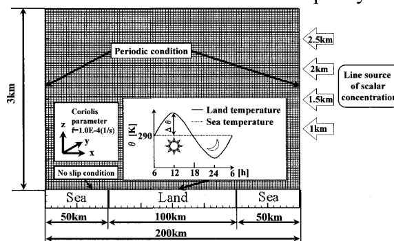
Fig.1 Schematic of computed area and calculating conditions
