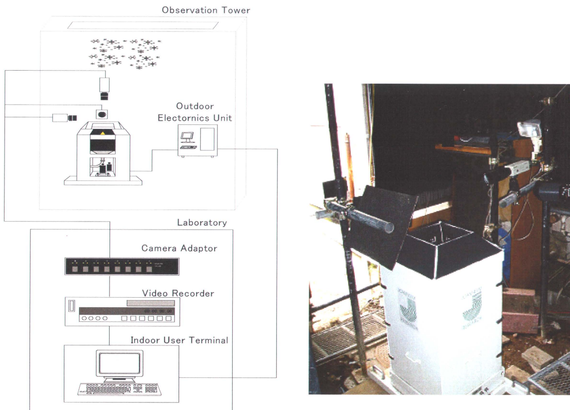
Fig.2 Measuring system.
