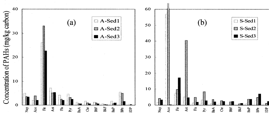
Fig. 4. Amount of PAHs bound to organic matter of different size fraction in sediment
