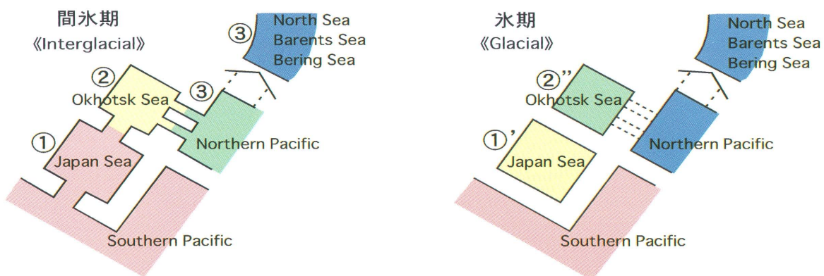
Marginal Sea Pumping Effect during glacial/interglacial periods
