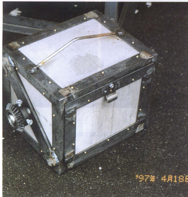
Figure 20 The separating device (upper) and the metal sieve – like tool which contaminated pebbles put in (down).
