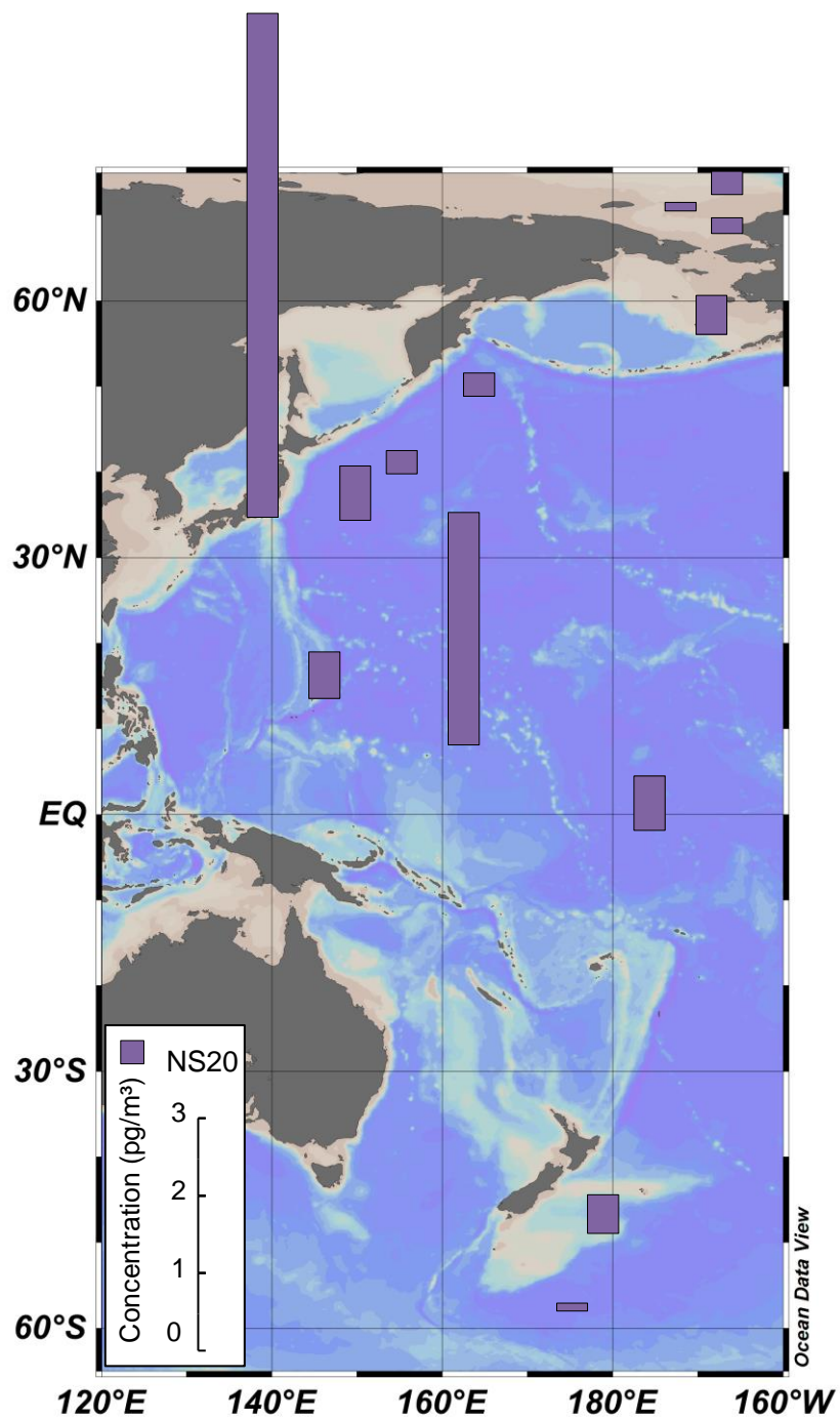
Figure 34 PFHxA concentration ( \text{pg m}^{-3} ) in air from NS20 sample. (Land sample in Japan is average PFOA concentration in roadside samples from Tsukuba ( n=10 ))
