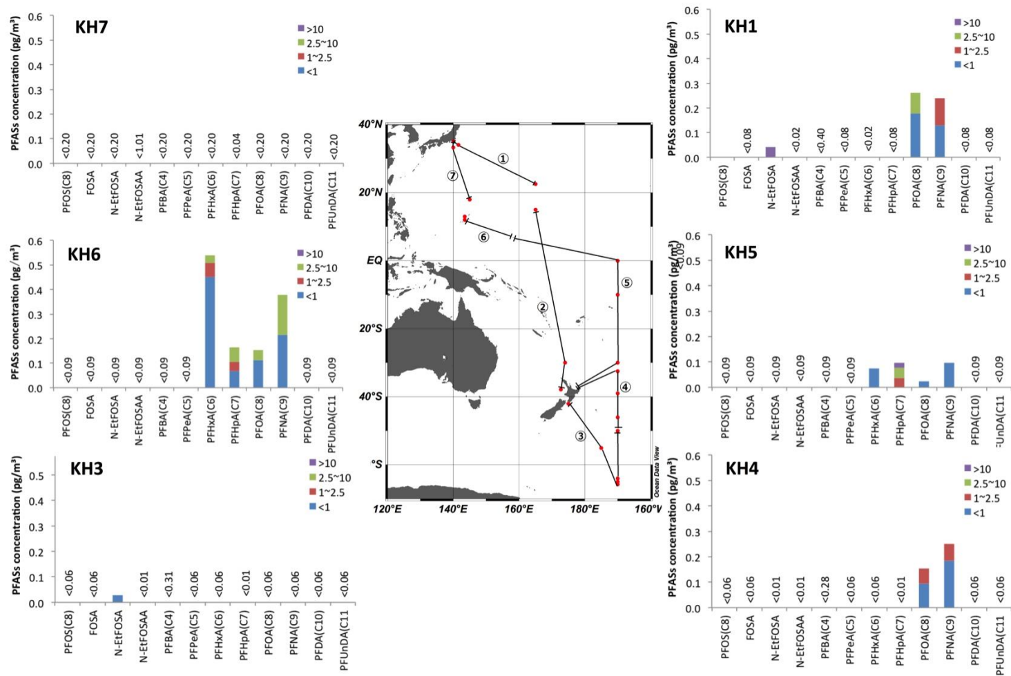
Figure 35 Selected PFASs concentration (pg m -3 ) in air from NS20 sample collected during cruise KH14-06.
