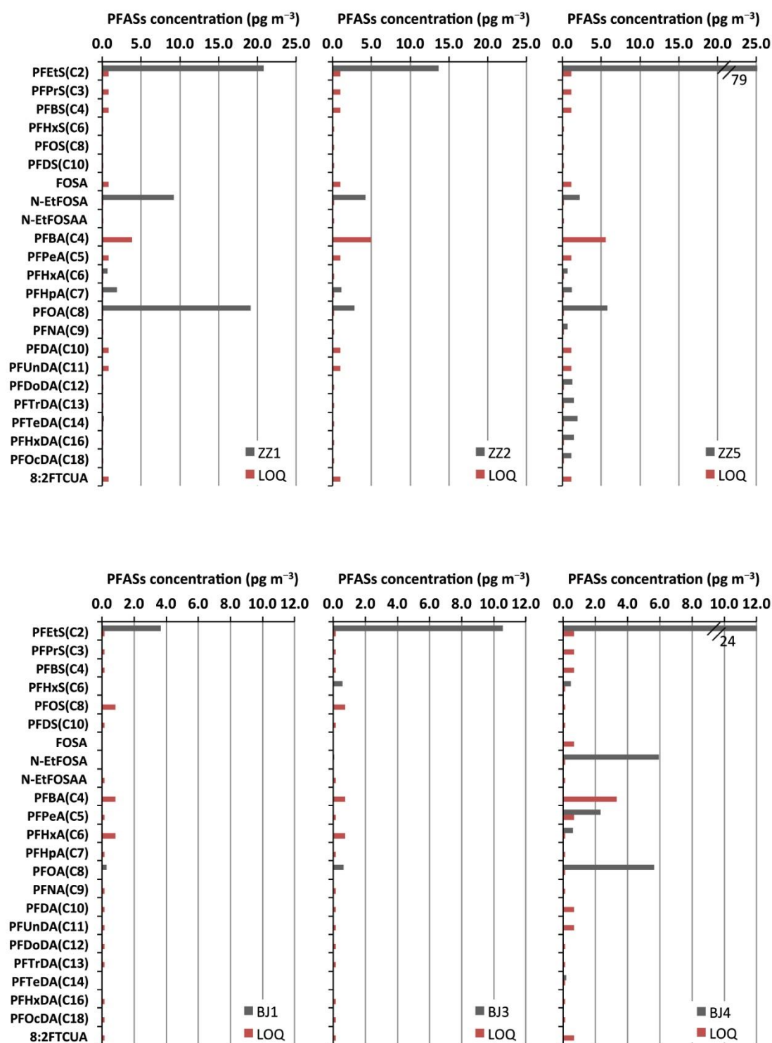
Figure 29 PFASs concentration in total particles ( \text{pg m}^{-3} ) for each sample.
