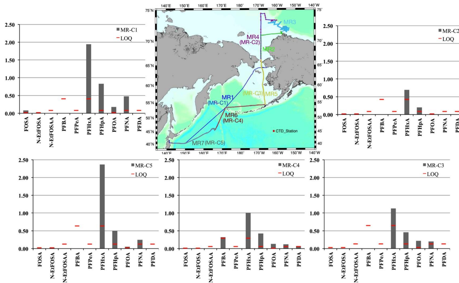
Figure 38 Selected PFASs concentration (pg m -3 ) in air from CMS sample collected during cruise MR15-03.
