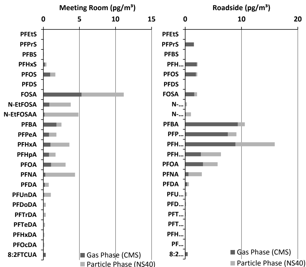
Figure 24 Average concentrations (pg m -3 ) of PFASs in particle phase (NS40) and gas phase (CMS) in meeting room (n=10) and roadside(n=9) air (error bar = standard deviation)
