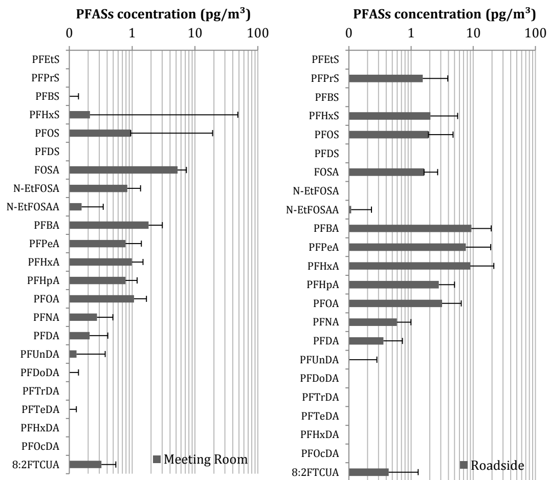
Figure 23 Average concentrations (pg m -3 ) of PFASs in gas phase(CMS) in meeting room (n=10) and roadside(n=9) air (error bar = standard deviation)
