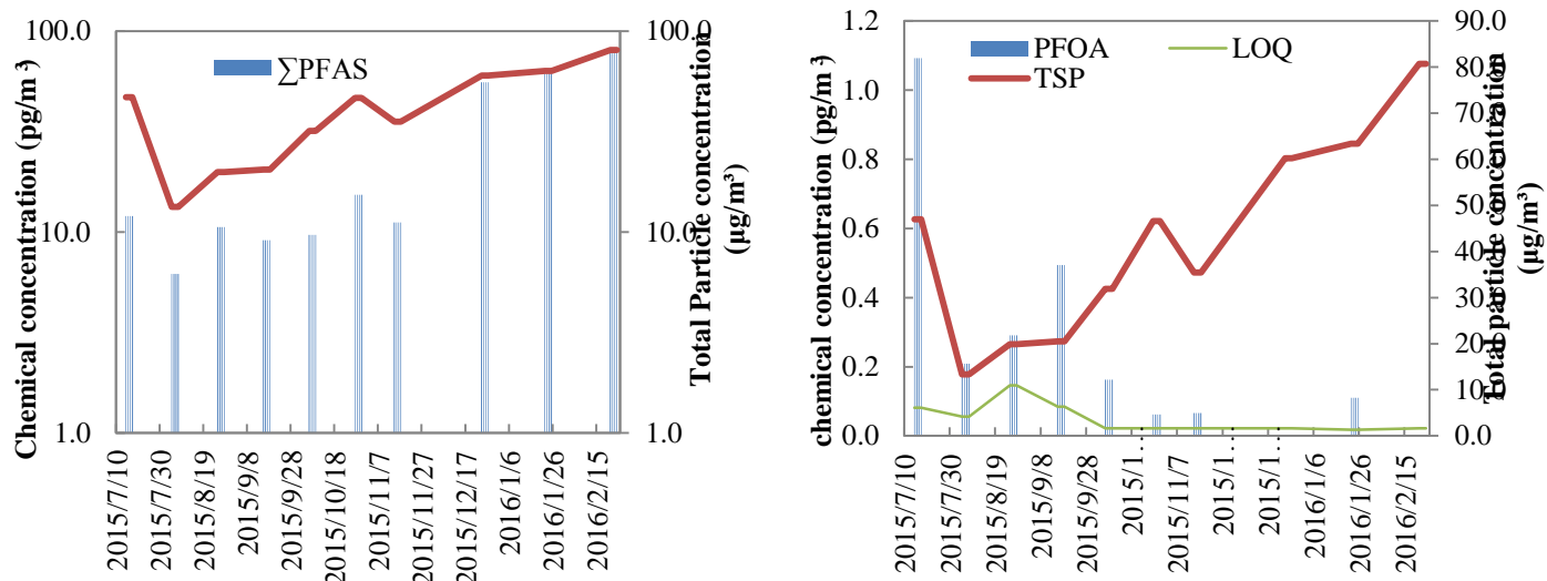
Figure 32 Time series of PFASs concentration (pg m -3 , primary y-axis) and total particle concentration (μg m -3 , secondary y-axis).
