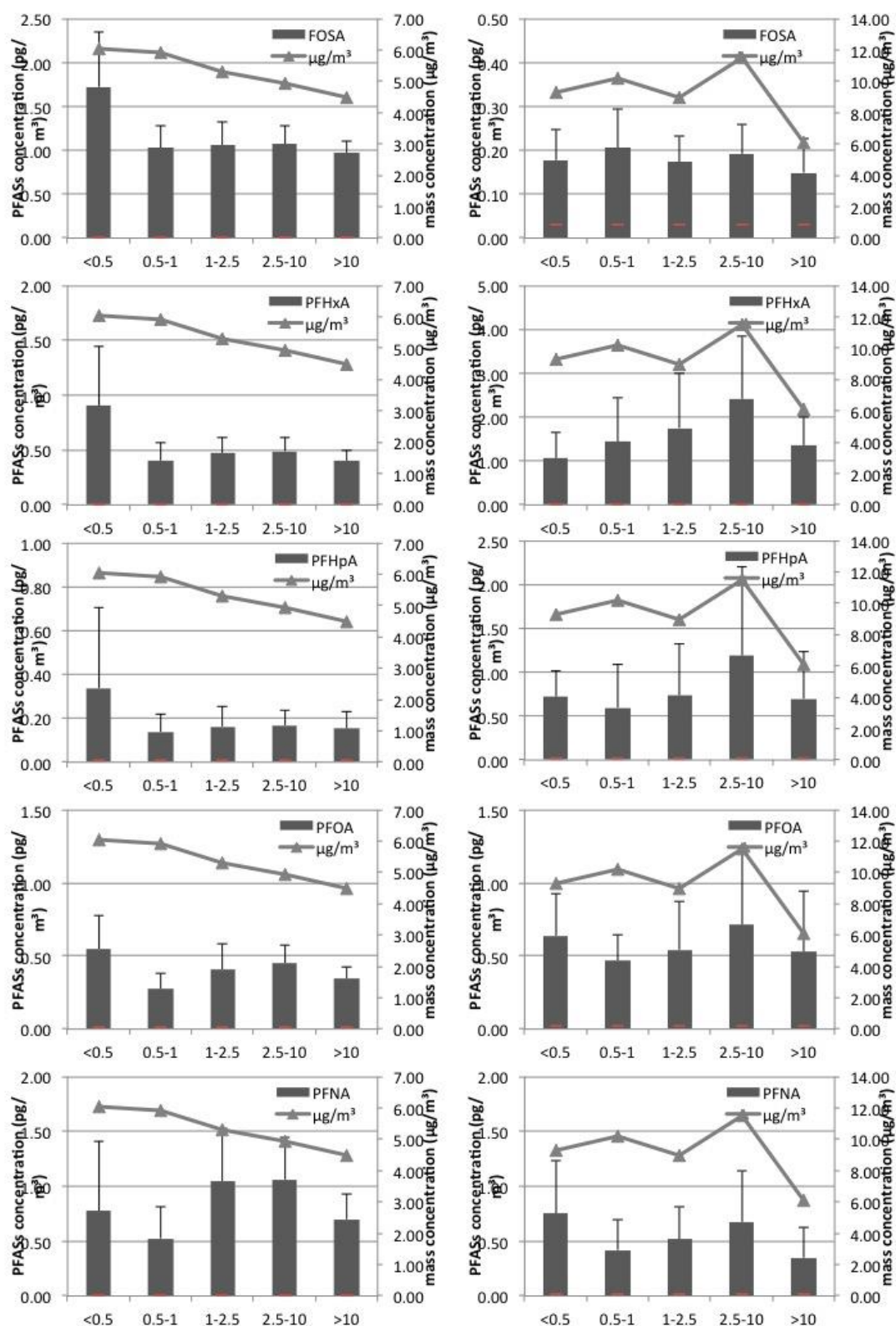
Figure 21 Size segregated concentrations (pg m -3 ) of selected PFASs and mass air concentration (μg m -3 ) in particulate matters from meeting room (left side, n=10) and
