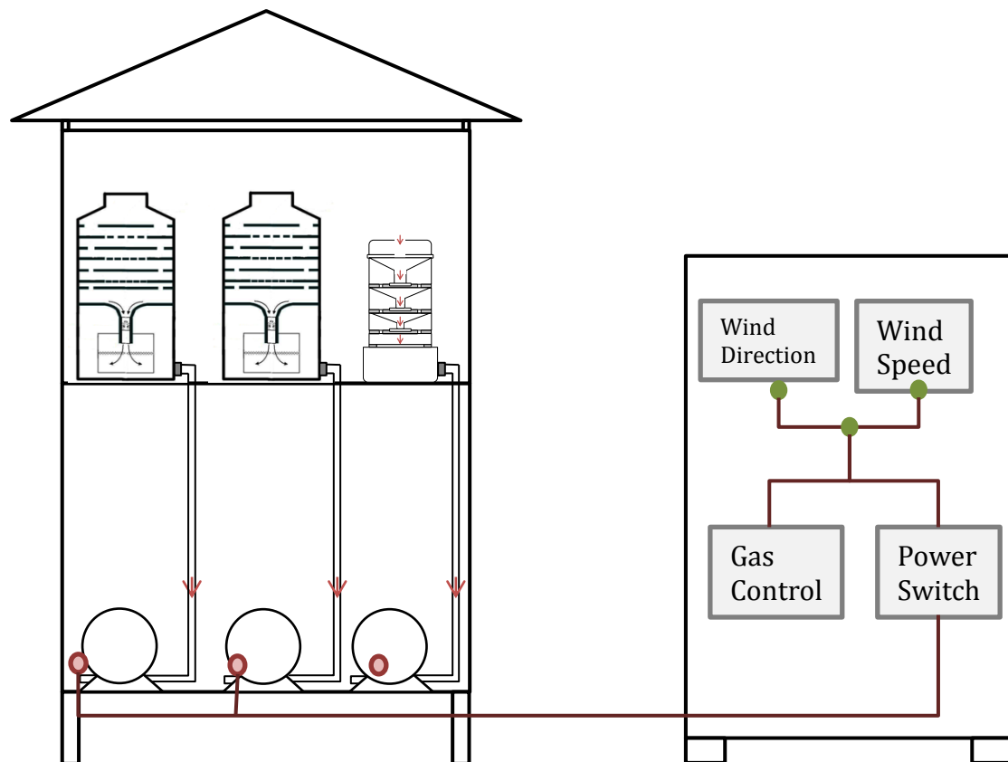
Figure 12 Schematic diagram of air sampling system on board
