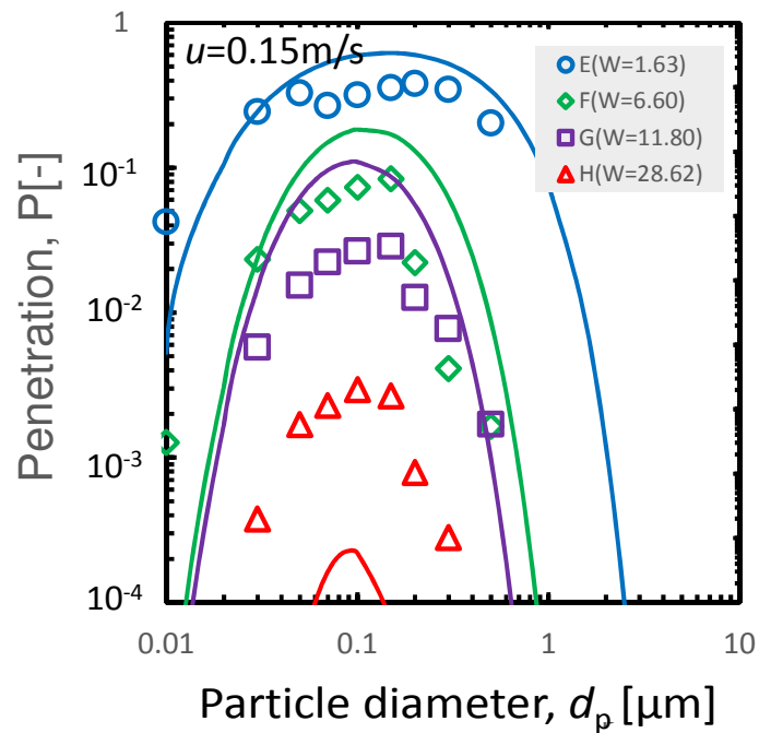
Fig. 2-24 Penetration of NaCl particles through sample E,F,G,H. ( u=0.15 m/s)
