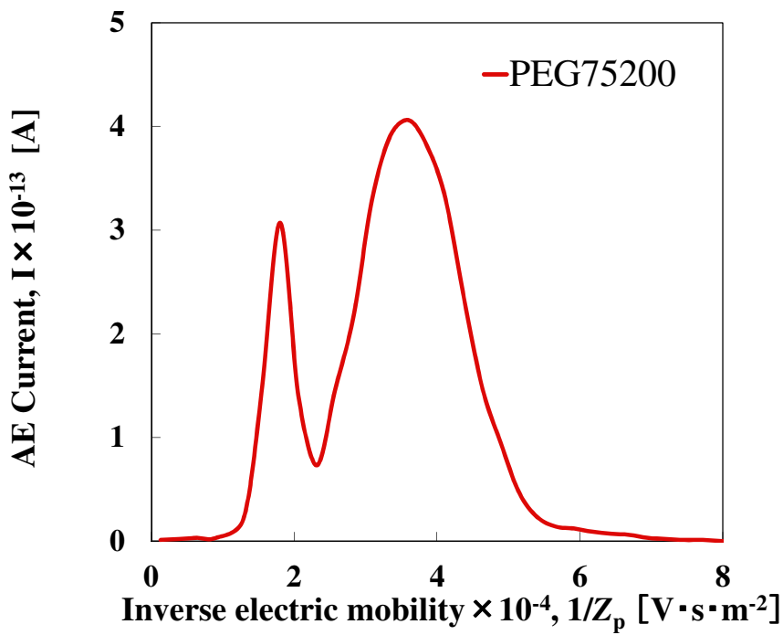
Fig. 3-20 Inverse mobility spectra of electrospayed PEG 75,200 (Without Am)
