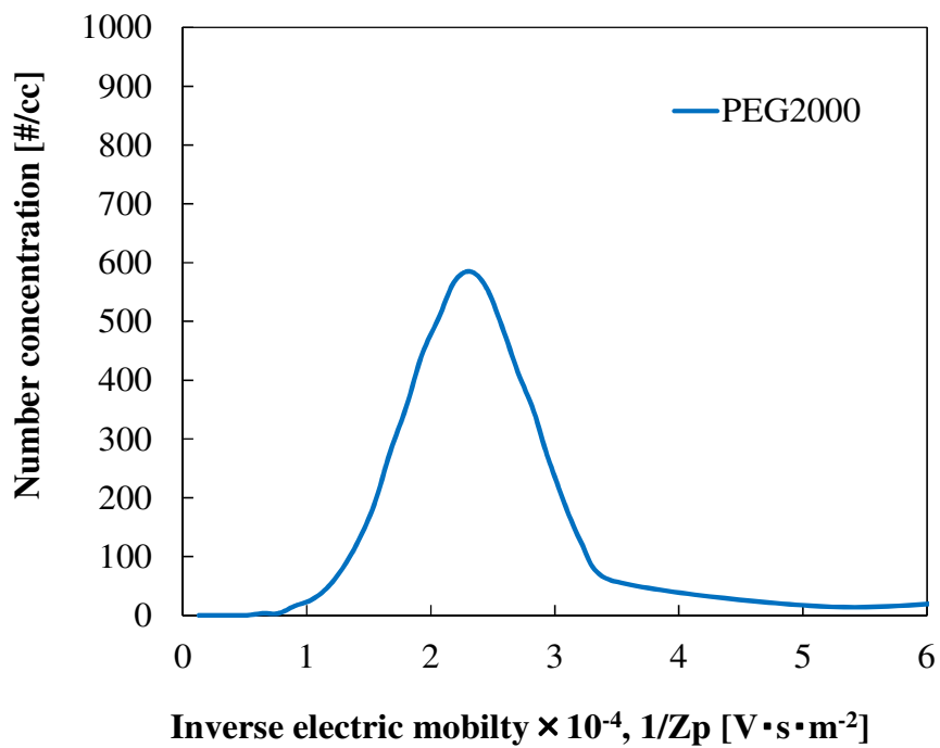
Fig. 3-10 Inverse mobility spectra of electrospayed PEG2000. (With Am)
