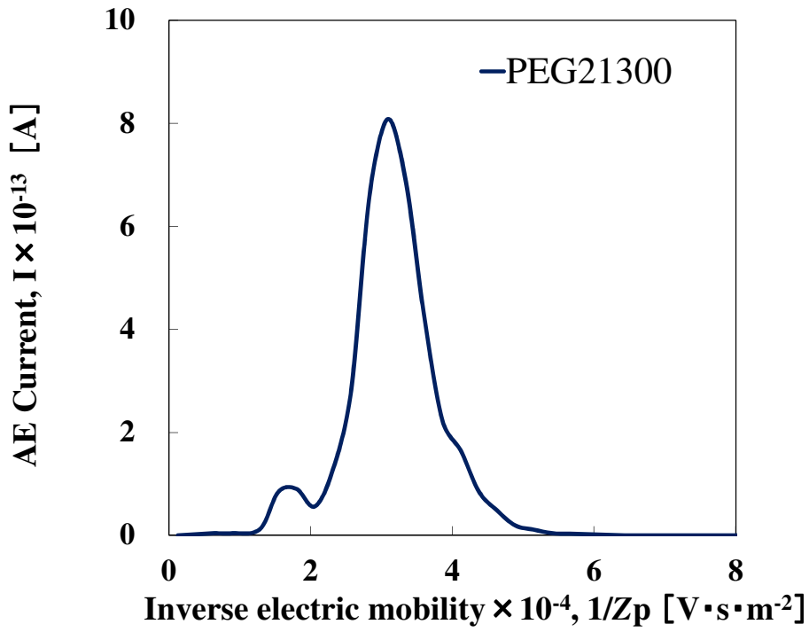
Fig. 3-19 Inverse mobility spectra of electrospayed PEG 21,300 (Without Am)
