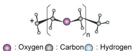
Fig. 3-5 Structure of Polyethylene glycol ion.
