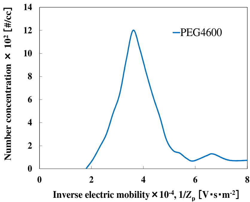
Fig. 3-8 Inverse mobility spectra of electrospayed PEG4,600 (With Am)
