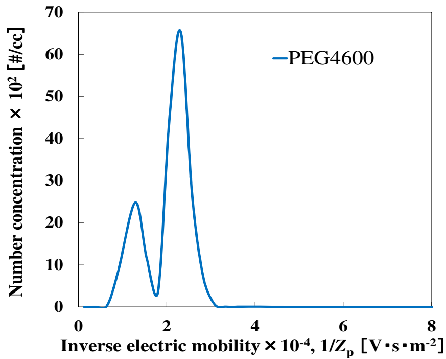
Fig. 3-7 Inverse mobility spectra of electrospayed PEG4.600 (Without Am)
