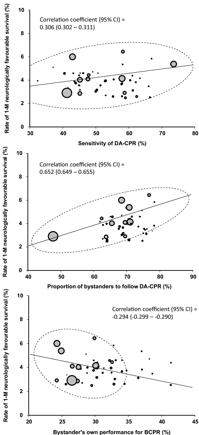
Fig. 2. Correlation between three DA-CPR- and BCPR-related indexes and OHCA survival. DA-CPR, dispatcher-assisted cardiopulmonary resuscitation; BCPR, bystander cardiopulmonary resuscitation. The size of each symbol reflects the number of out-of-hospital cardiac arrests in each prefecture. Bivariate normal density ellipsoid ( \alpha = 0.95 ) was presented.
