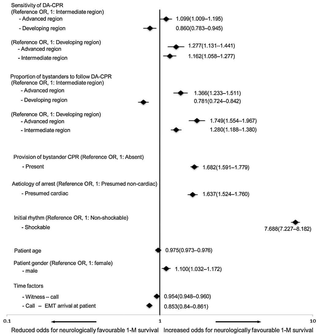
Fig. 3. Multivariable logistic regression analysis for survival. DA-CPR, dispatcher-assisted cardiopulmonary resuscitation; CPR, cardiopulmonary resuscitation; EMT, emergency medical technician. Multiple logistic regression analysis was used to examine the association between neurologically favourable 1-M survival, OHCA backgrounds, and regional classification based on BCPR and EMS-related indexes. We sequentially introduced groups of variables into the model: first, basic variables known to be associated with OHCA outcomes, then variables identified as significant in the univariable analysis in a stepwise manner to obtain the lowest Bayesian information criterion (BIC). The generalized R^2 of the final model was 0.2559.
