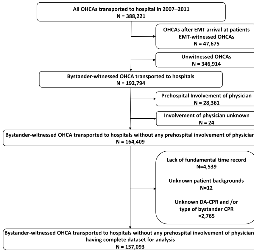
Fig. 1. Overview of nationwide data collection and selection. OHCA, out-of-hospital cardiac arrest; DA-CPR, dispatcher-assisted cardiopulmonary resuscitation; CPR, cardiopulmonary resuscitation.
