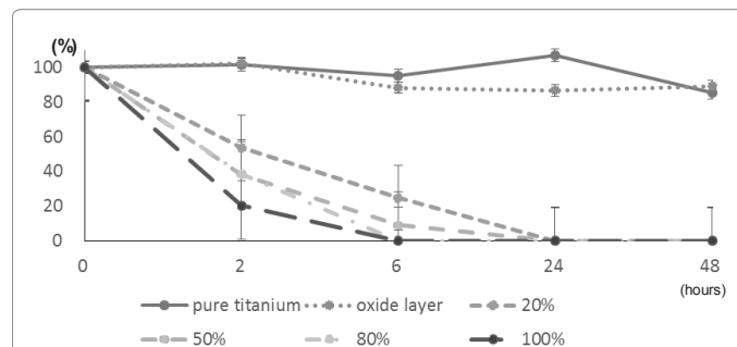
Figure 6: In vitro antibacterial activity of titanium implants with different iodine contents on S. aureus . While pure titanium implants and 0% iodine implants had no antibacterial activity, implants with \geq 20\% iodine showed a significant decrease in the number of colonies compared with the control group beginning at 2 hours ( p < 0.05 ). Implants with 100% iodine exhibited significantly greater and faster decreases in the number of colonies compared to 20% iodine implants ( p < 0.05 ). Implants with \geq 20\% iodine showed complete inhibition of bacterial colonies after 24 hours.
