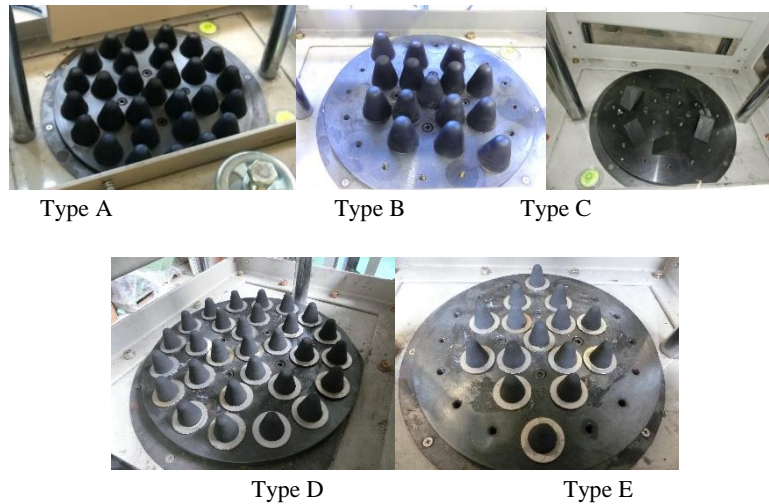
Figure 2: Rubber cushion
