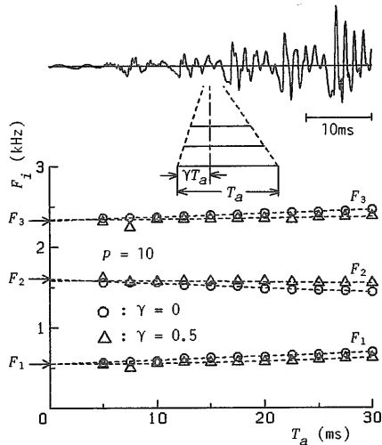
図4 極周波数推定値の分析窓長 T_a 依存性—合成有声破裂音/ga/— Fig. 4 The T_a (window length) —dependency of pole frequency estimation for a synthetic syllable /ga/.
