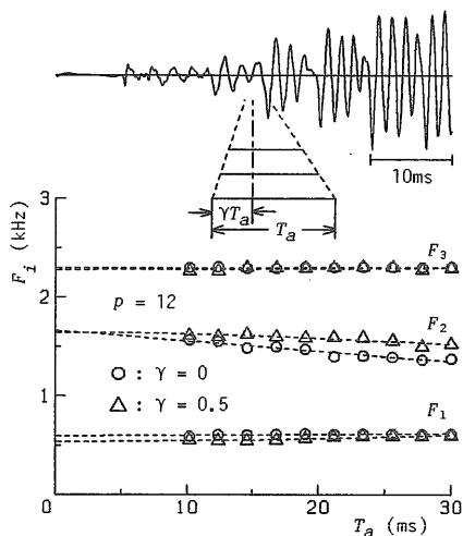
図7 極周波数推定値の分析窓長 T_a 依存性—自然有声破裂音/ga/— Fig. 7 The T_a (window length) —dependency of pole frequency estimation for a natural syllable /ga/.
