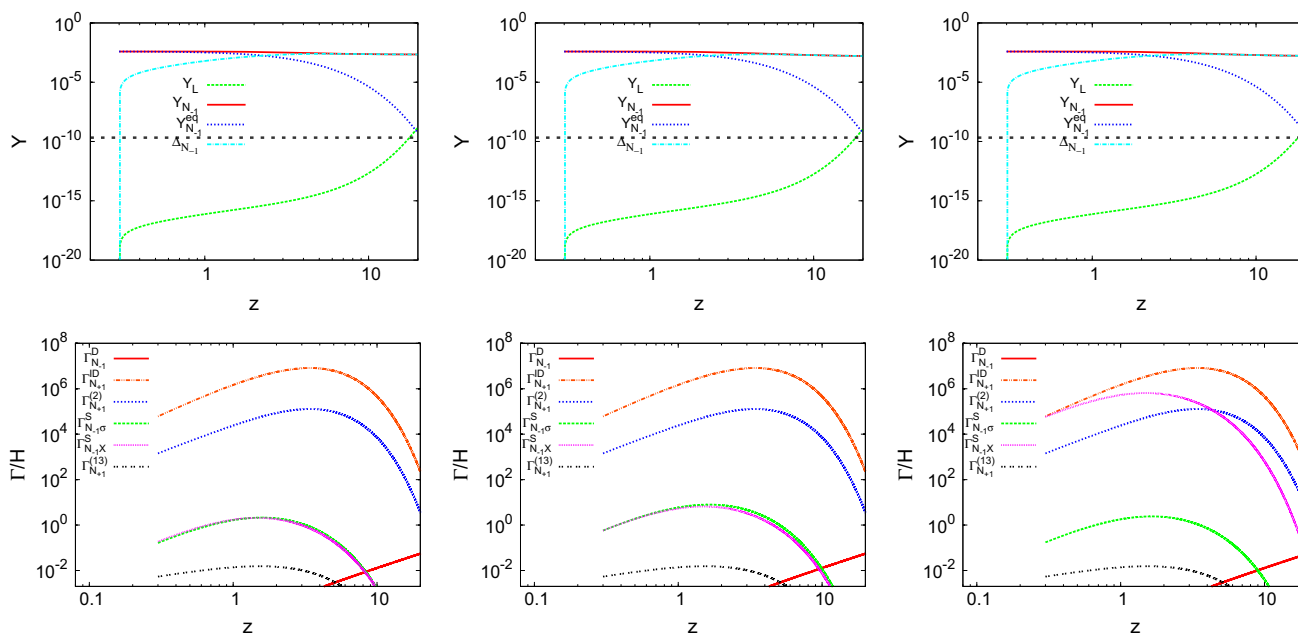
Fig. 2 In the upper panels , solutions of the Boltzmann equations are plotted as a function of z for the case A shown in Table 1. In the lower panels , relevant reaction rates \Gamma/H are plotted as a function of z for the same parameters used in the corresponding upper panels . Reaction rates of the \mathcal{N}_{-1} decay, the \mathcal{N}_{+1} inverse decay, and the lep-
