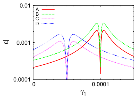
Fig. 1 CP asymmetry as a function of \gamma_1 for typical values of (|y_1|, |h_{\alpha 1}|) . In each case, these parameters are fixed as A( 10^{-5}, 4 \times 10^{-4} ), B( 10^{-5}, 5 \times 10^{-4} ), C( 2 \times 10^{-5}, 4 \times 10^{-4} ), and D( 2 \times 10^{-5}, 5 \times 10^{-4} ). Other relevant parameters are taken to be \tilde{\gamma}_1 = 0.1, \tilde{y}_1 = 10^{-8}, M_1 = \langle S \rangle = 2 \text{ TeV} and M_\eta = 1 \text{ TeV}
