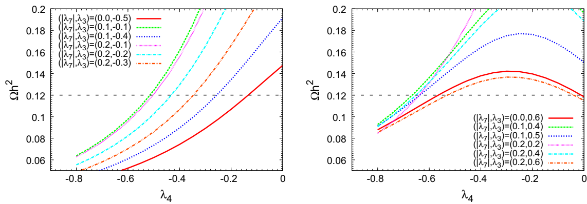
Fig. 3 Relic abundance of \eta_R in the case of the existence of new interactions. It is plotted as a function of \lambda_4 for typical sets of (|\lambda_7|, \lambda_3) . In the left and right panels, \lambda_3 is assumed to be negative and positive,
