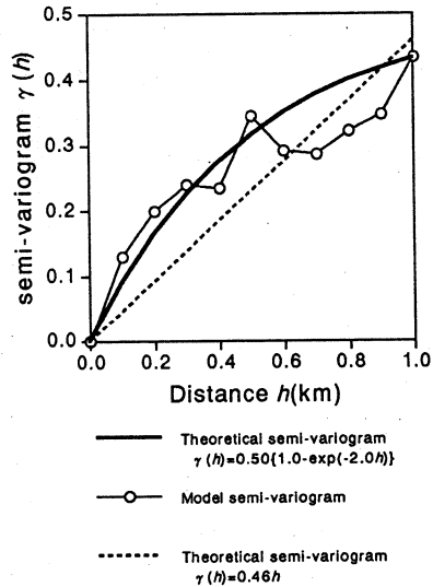
Fig.4 Semi-variogram
