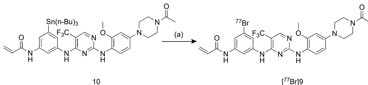
Scheme 2. Radiosynthesis of compound [^{77}\text{Br}]9 . (a) [^{77}\text{Br}]\text{Br}^- , acetic acid, NCS, ethanol, 80\text{ }^\circ\text{C} , 60 min.
