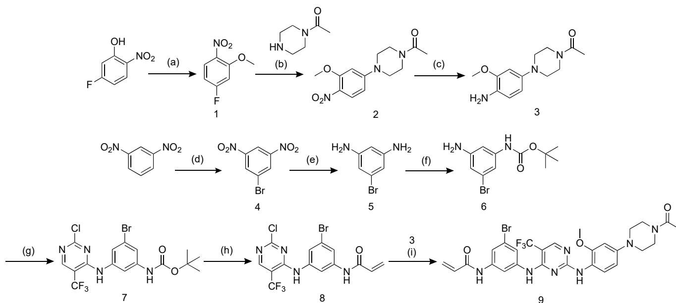
Scheme 1. Synthesis of non-radioactive brominated CO-1686. (a) K_2CO_3 , CH_3I , acetone, 0\text{ }^\circ\text{C} , 5 h; (b) DIPEA, DMA, 90\text{ }^\circ\text{C} , overnight; (c) Pd/C 10%, H_2 , MeOH, rt, 5 h; (d) H_2SO_4 , NBS, 80\text{ }^\circ\text{C} , 1.5 h; (e) SnCl_2 \cdot 2H_2O , ethanol, rt, 3 h; (f) Boc_2O , MeCN, 50\text{ }^\circ\text{C} , overnight; (g) 2,4-dichloro-5-(trifluoromethyl) pyrimidine, DIPEA, n -butanol, 0\text{ }^\circ\text{C} , 2 h, rt, 4 h; (h-1) HCl/ethyl acetate, rt, 1 h; (h-2) acryloyl chloride, DIPEA, dichloromethane, -30\text{ }^\circ\text{C} to rt, 2 h; (i) TFA, 1,4-dioxane, 60\text{ }^\circ\text{C} , 3 h.
