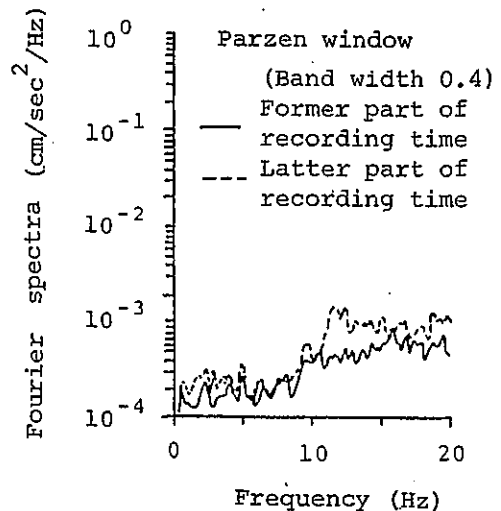
Fig. 5 Fourier spectra of microtremor records
