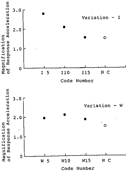
Fig. 3 Magnification of response acceleration in relation to interval and width of gravel piles.
