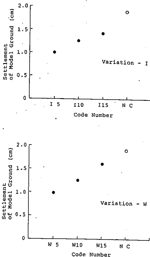
Fig. 7 Settlement of model ground at inside part in relation to interval and width of gravel piles.
