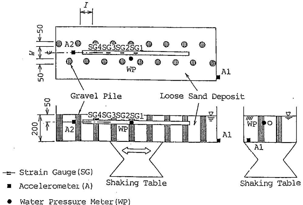
Fig. 1 General view of test apparatus (mm).
