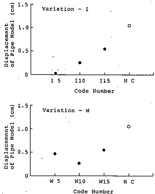
Fig. 8 Displacement of pipe model in relation to interval and width of gravel piles.
