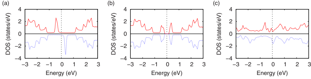
FIG. 2. (Color online) DOS of freestanding ZGNRs having the (a) PIES and (b) APIES states, respectively. The PDOS of the ZGNR on Ni(111) is shown in (c). The energy is measured from the Fermi energy. The solid and dashed lines denote the up-spin and down-spin states, respectively.
