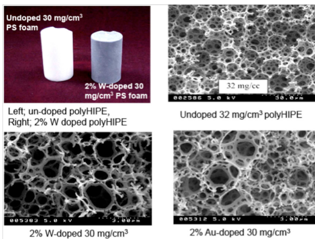
FIG. 6. SEM images of un-doped and doped W and Au polyHIPEs. Reprinted with permission from Steckle and Nobile, Fusion Sci. Technol. 43 , 301 (2003). Copyright 2007 American Nuclear Society. 81
