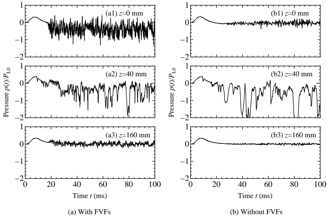
Fig. 4 Instantaneous pressure p(t) = P(t) - P_{\text{atm}} in the glottal flow for P_{L0} = 800 Pa.
