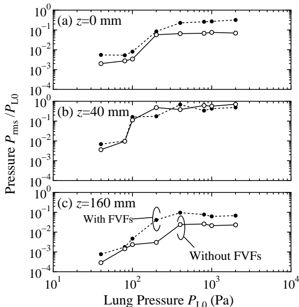
Fig. 6 Root-mean-square of the pressure fluctuation P_{\text{rms}} with respect to the lung pressure P_{L0} .
