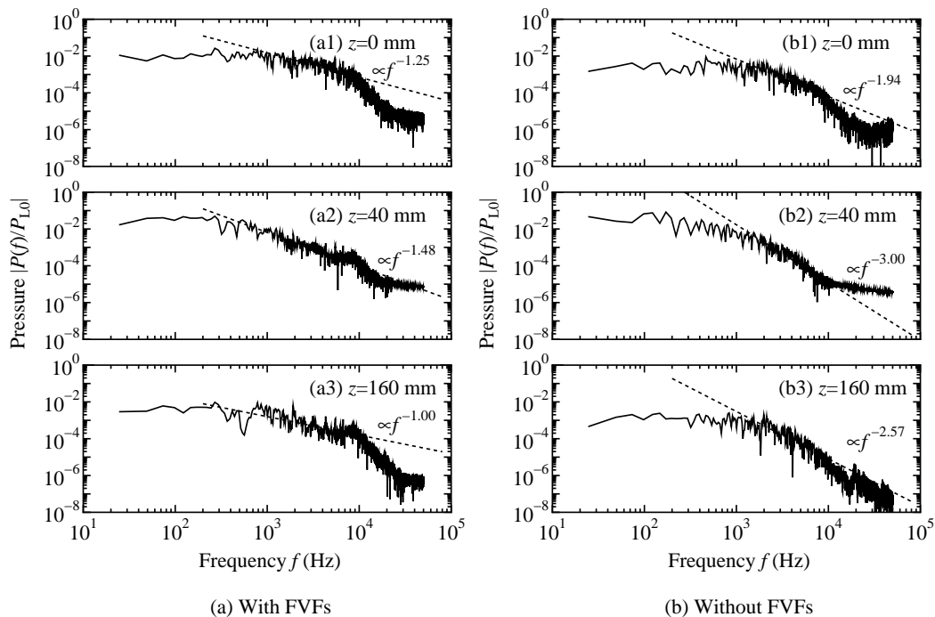
Fig. 5 Frequency spectra of pressure in the unsteady glottal flow at P_{L0} = 800 Pa. These results correspond to the pressure in Fig. 4. The dashed curves are fitting curves using a function |P(f)| \propto f^{-\alpha} with \alpha ranging from 1 kHz to 10 kHz.
