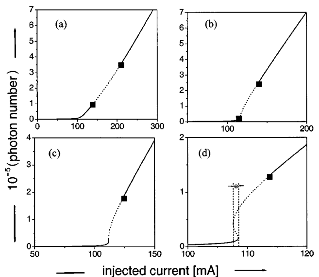
FIG. 5. Dependence of stationary photon number S on the injected current for different values of the carrier lifetime in the saturable absorber. The cavity length is 650\ \mu\text{m} and the carrier lifetime is (a) \tau_s(\text{SA}) = 0.1\text{ ns} , (b) \tau_s(\text{SA}) = 1.0\text{ ns} , (c) \tau_s(\text{SA}) = 1.4\text{ ns} , (d) \tau_s(\text{SA}) = 2.0\text{ ns} . The thickness of the saturable absorber is 2 nm. The other parameters are as in Table I. The squares represent the Hopf-bifurcation points. In the range “e” the laser shows excitable behavior.
