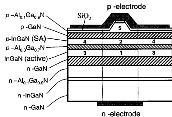
FIG. 1. Schematic illustration of the blue-violet InGaN laser with a saturable absorber incorporated.
