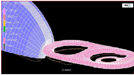
Fig.13 Finite element analysis model.
