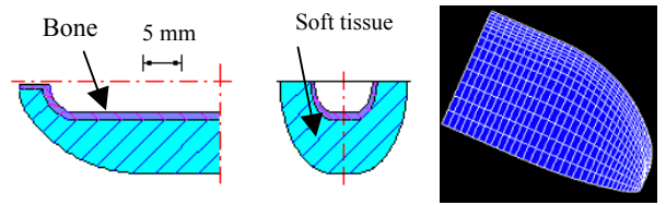
Fig. 8 Model of distal part of index finger.
