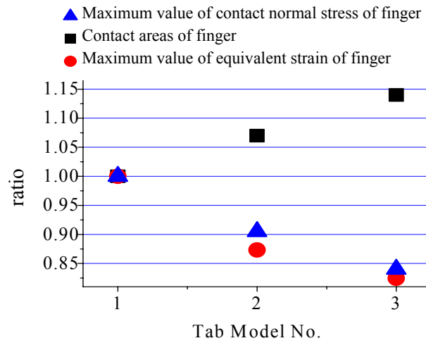
Fig.16 Comparison of three tab models.
