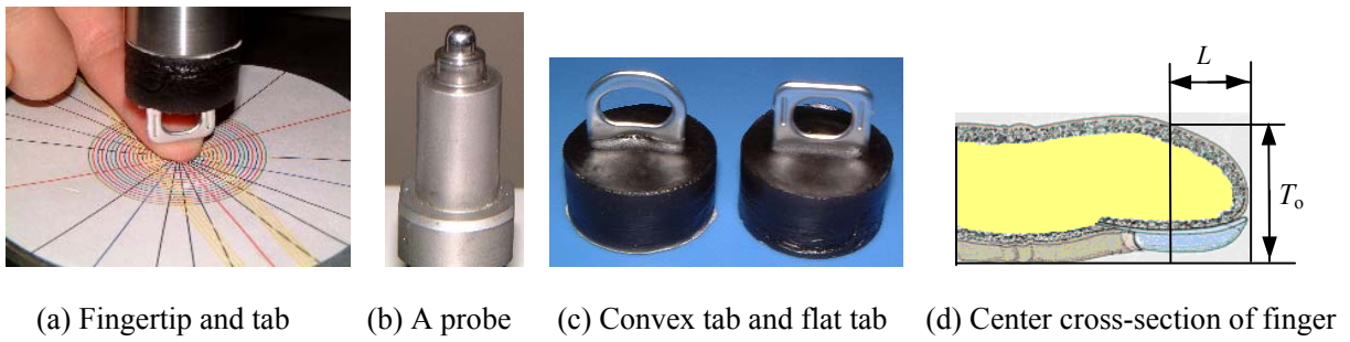
Fig.2 Experimental setup.
