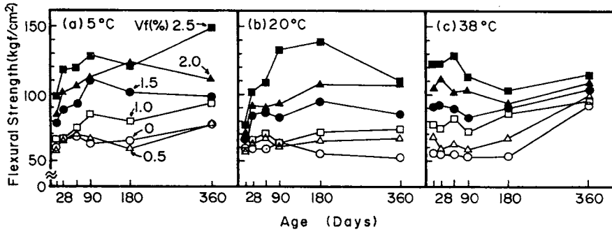
Fig.6 Flexural strength of glass fiber reinforced mortars with flyash.
