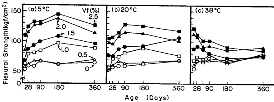
Fig.7 Flexural strength of glass fiber reinforced mortars with silica fume.
