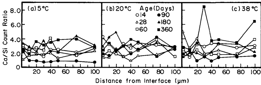
Fig. 12 Ca/Si count ratio in the interfacial region in the flyash-bearing cement paste.
