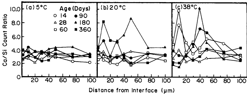
Fig.5 Ca/Si count ratio in the interfacial region in the admixture-free cement paste.
