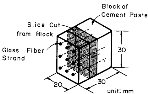
Fig. 1 Schematic diagram of a specimen for microhardness measurement and EDXA analysis.
