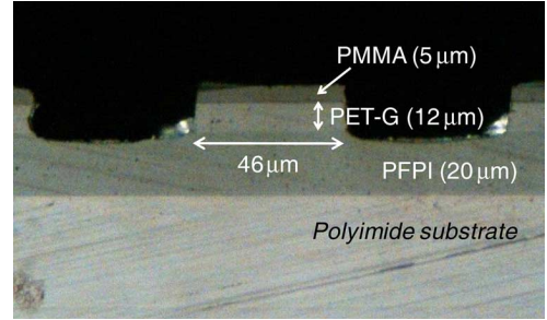
Fig. 3. Photograph of the facet of the PET-G channel waveguide.
