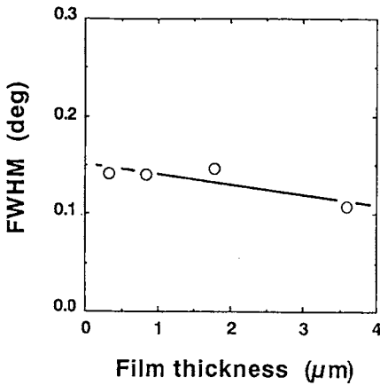
Fig.5 The dependence of the FWHM of the perovskite (100)/(001) peak on film thickness.
