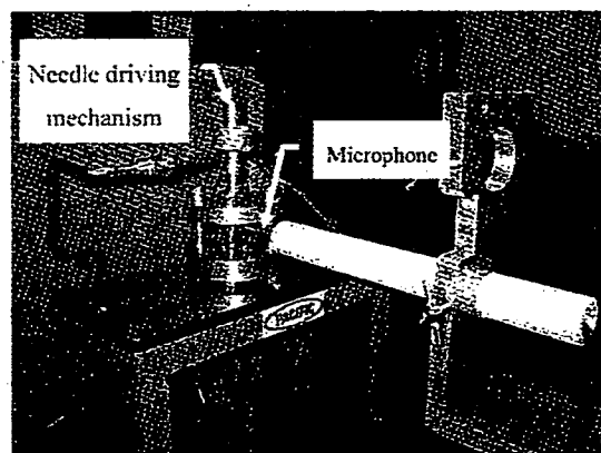
Fig.6 Acoustic noise measurement
