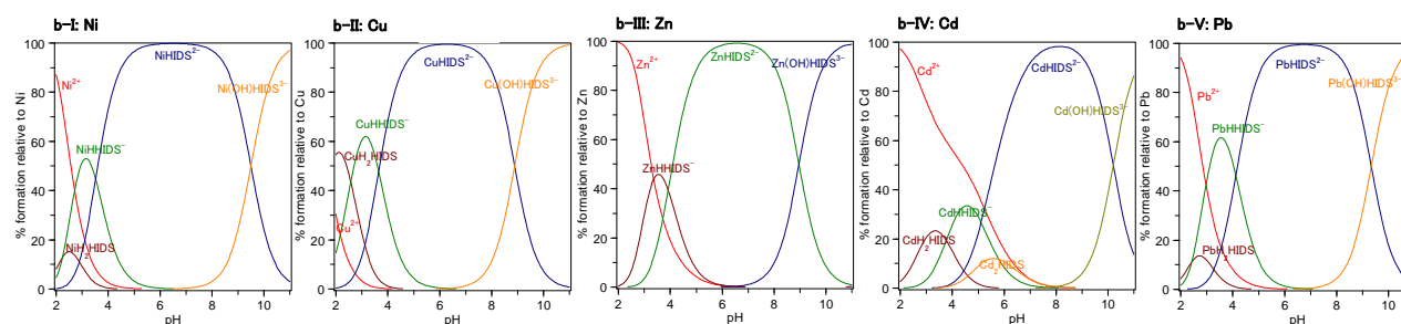
Figure 5. The species distribution curves for M(II) + L (M = Ni, Cu, Zn, Cd, Pb; L = GLDA or HIDS) in the aqueous medium at the ionic strength, I = 0.1 \text{ mol} \cdot \text{dm}^{-3} and at 25 \pm 0.1^\circ\text{C} .
