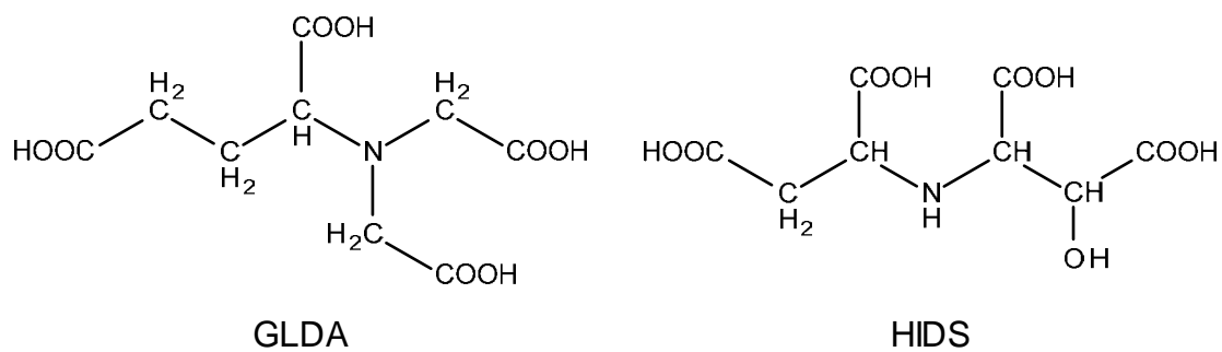
Figure 1. The chemical structures of DL-2-(2-carboxymethyl)nitrilotriacetic acid (GLDA) and 3-hydroxy-2,2'-iminodisuccinic acid (HIDS).
