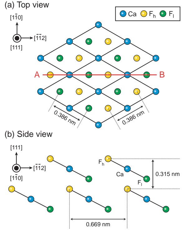
Fig. 1 Crystal structure of fluorite(111) surface. (a) Top view. (b) Side view.
