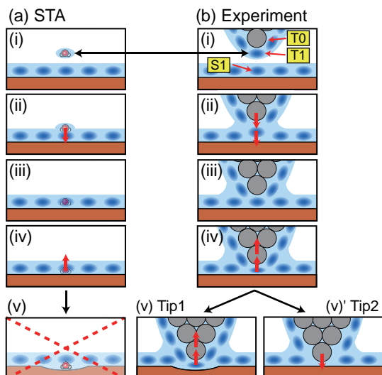
Fig. 5 Schematic models showing relationship between a tip position and a measured force in (a) the STA model and (b) a real experiment.
