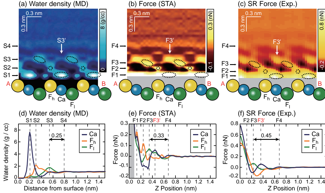
Fig. 3 z cross sections of the (a) \rho(\mathbf{r}) , (b) F_{STA}(\mathbf{r}) and (c) F_{exp}(\mathbf{r}) images. z profiles of the (d) \rho(\mathbf{r}) , (e) F_{STA}(\mathbf{r}) and (f) F_{exp}(\mathbf{r}) images over Ca, F_h and F_l sites.
