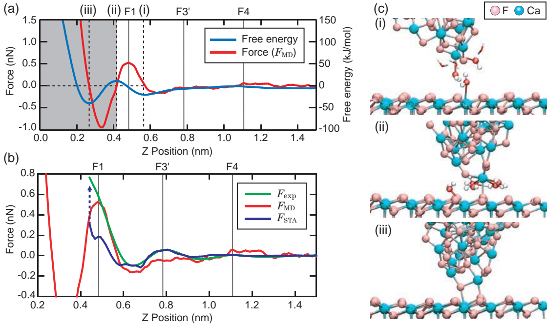
Fig. 4 (a) Free energy and F_{MD}(\mathbf{r}) profiles over a Ca site obtained by MD simulation. (b) F_{MD}(\mathbf{r}) , F_{STA}(\mathbf{r}) and F_{exp}(\mathbf{r}) profiles over a Ca site. (c) Snap shots of the MD simulation model for z tip positions (i)-(iii) indicated in (a).
